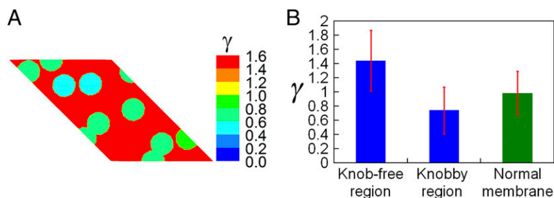
Fig. 5. Stiffening due to the inhomogeneous strain induced by the presence of the knobs ( \alpha=0.35 ). (A) Inhomogeneous shear strain distribution in the spectrin network. The shear strain in the knob-free regions is much higher than that applied, representing a stiffening mechanism due to the strain-hardening property of the spectrin network. (B) The average shear strain in the knob-free regions is \gamma_F=1.44 , whereas that in the knobby regions is \gamma_K=0.74 at an applied shear strain \gamma_C=1 . The shear strain in the normal spectrin network (without knobs) is homogeneous and consistent with the applied shear strain.
